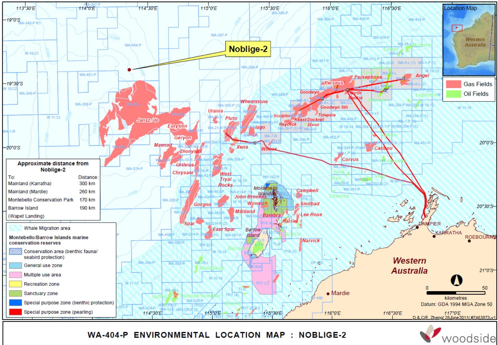
Figure 2-1: Drilling Location Map for Noblige-2 Appraisal Well
