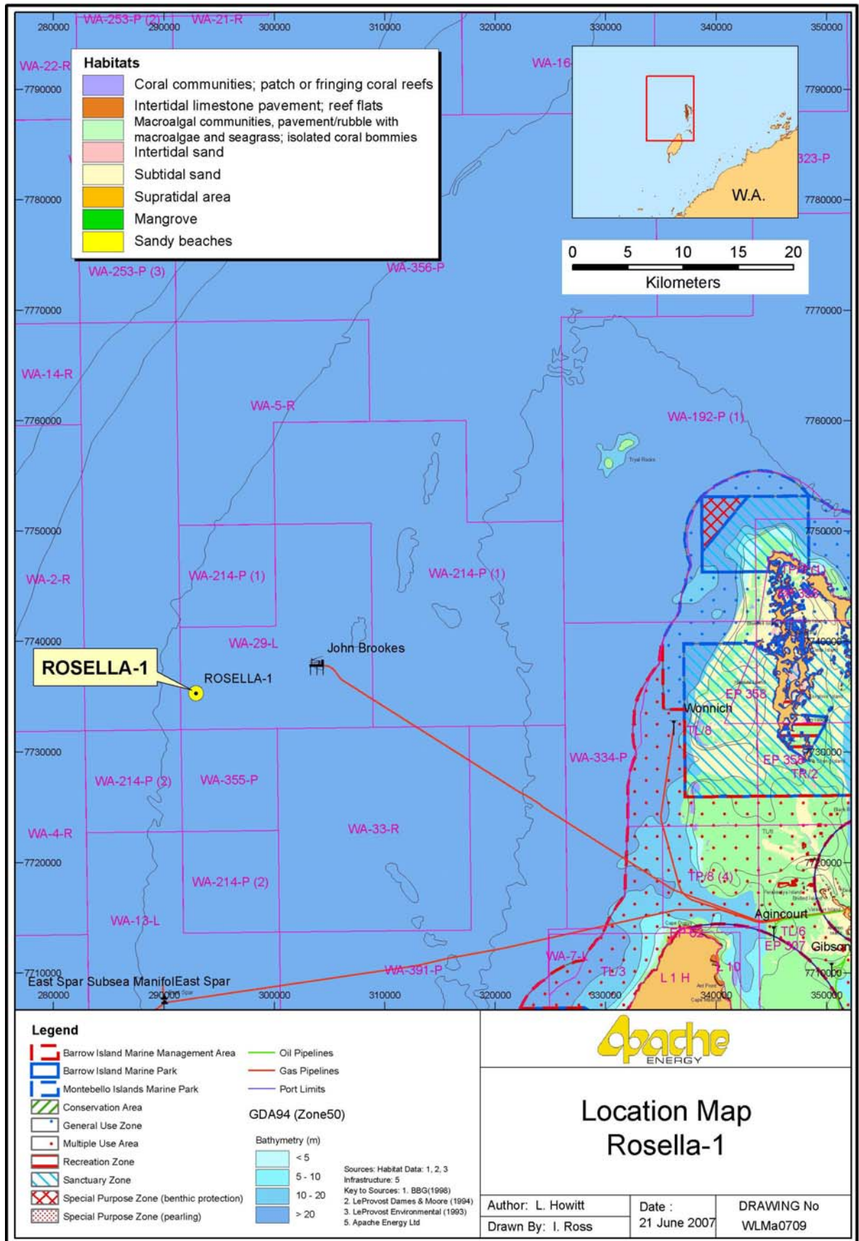
Figure 1 Location of the Rosella-1 drill site
