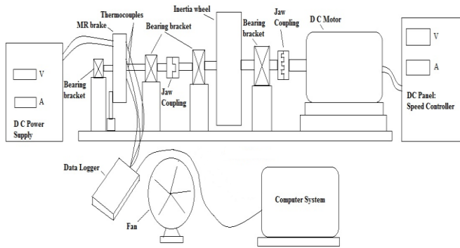
Fig 11.Schematic diagram of the MR brake test rig
