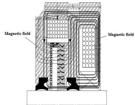
Fig 10. Iron particle chain after compression
