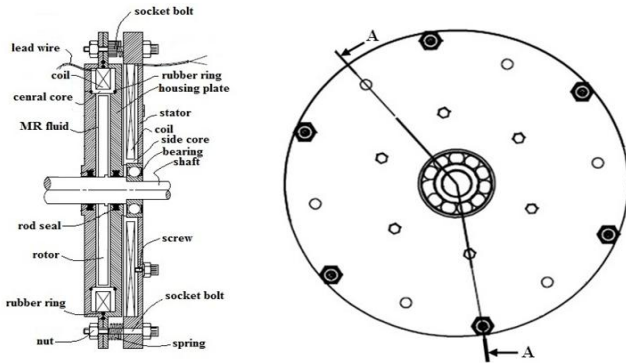
Fig 6. Schematic drawing of MR brake
