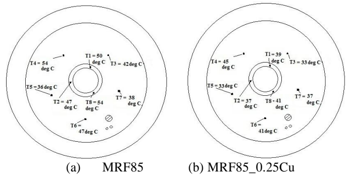
(a) MRF85 (b) MRF85_0.25Cu Fig 23. Thermocouple readings using MRF85 and MRF85_0.25Cu at 600 RPM
