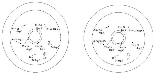
(a) MRF85_0.50Cu (b) MRF85_0.75Cu Fig 22. Thermocouple readings using MRF85_0.50Cu and MRF85_0.75Cu at 200 RPM
