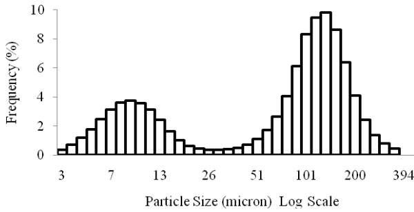
Fig 1. Probability volume density graph of particle sizes First MR fluid sample MRF85 contains 14.5% by wt silicone oil, 0.5% by wt oleic acid, and 85% by wt carbonyl iron powder as indicated in Table 1. Similarly three other MR fluid samples contain 0.5% by wt oleic acid, 85% by wt carbonyl iron powder, specification of which is listed in Table 1.
