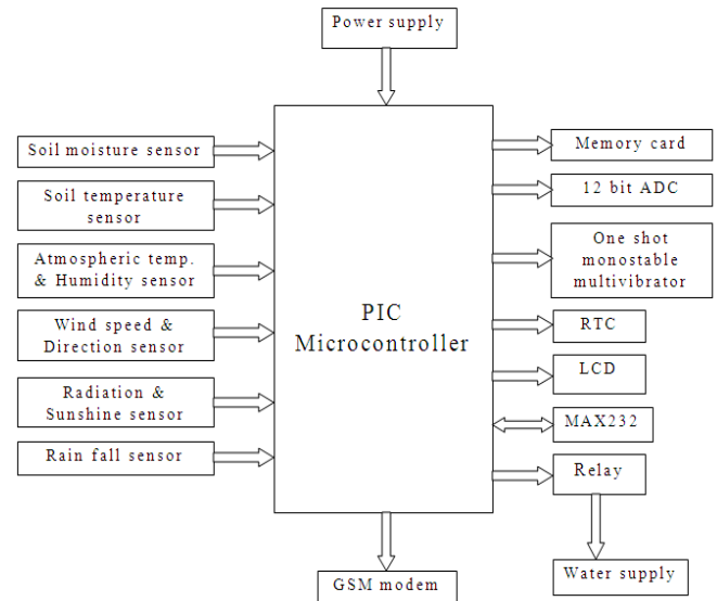
Figure 2.1 System Block Diagram
