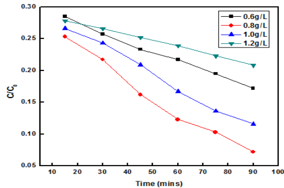
Figure 6 Effect of catalyst weight
