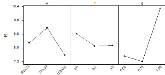
Main Effects Plot - Data Means for R
