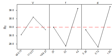
Main Effects Plot - Data Means for Rx
