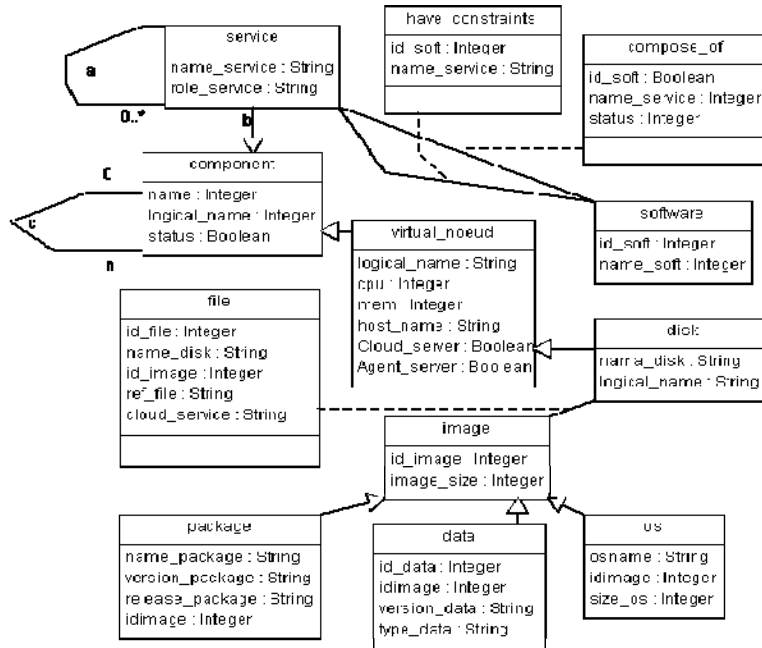
Fig 1: Meta data model for deployment in the cloud [1]
