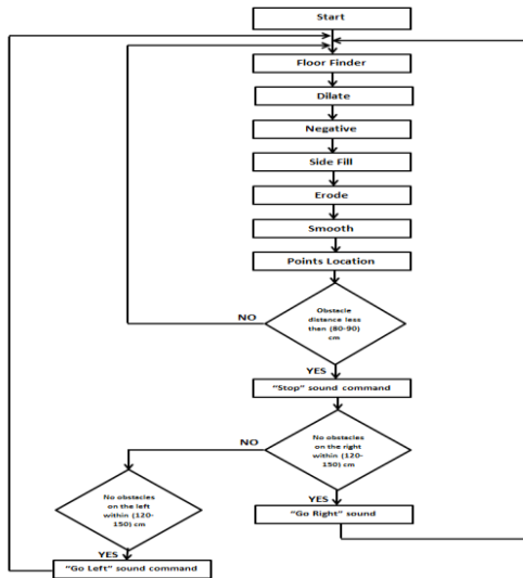
Figure 9: RoboRealm Flow chart
