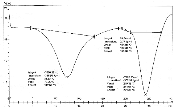
Fig 4 . DSC Thermogram of Polyacrylamide
