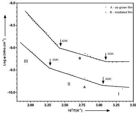
Fig 3. Electrical conductivity in Polyacrylamide
