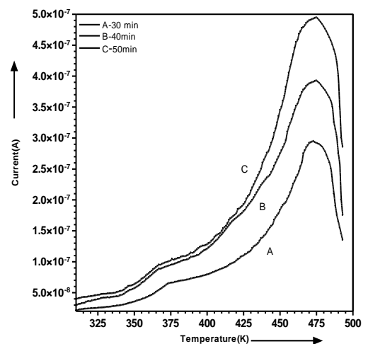
Fig 2. Thermally stimulated current (TSC) spectra of Polyacrylamide
