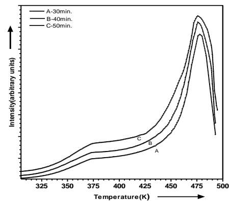
Fig 1. Thermally stimulated luminescence (TSL) spectra of Polyacrylamide
