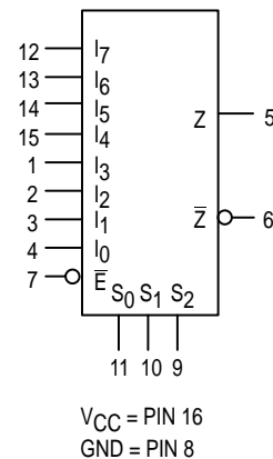
LOGIC SYMBOL
