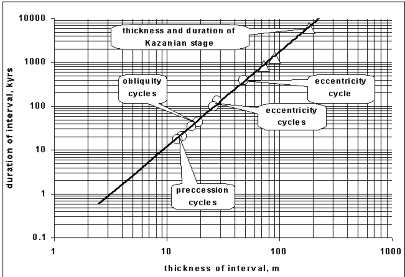
Figure 5. Duration of intervals (cycles) plotted against their thickness on logarithmic scale.
