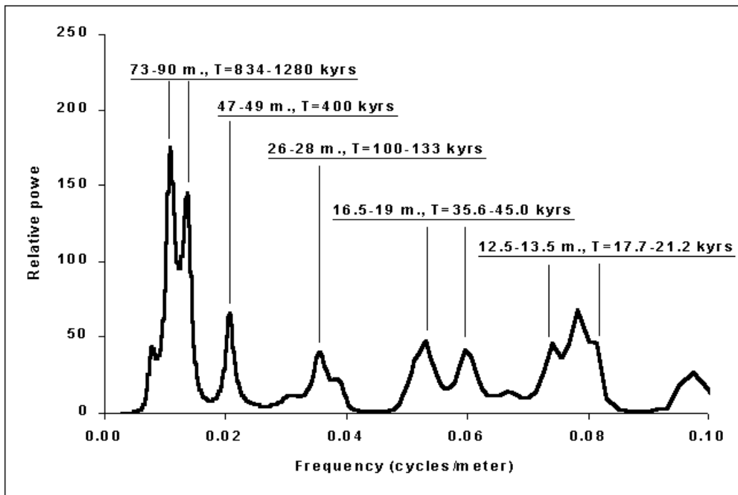
Figure 4. The generalized spectra from all well sections, showing lengths of cycles and their duration.
