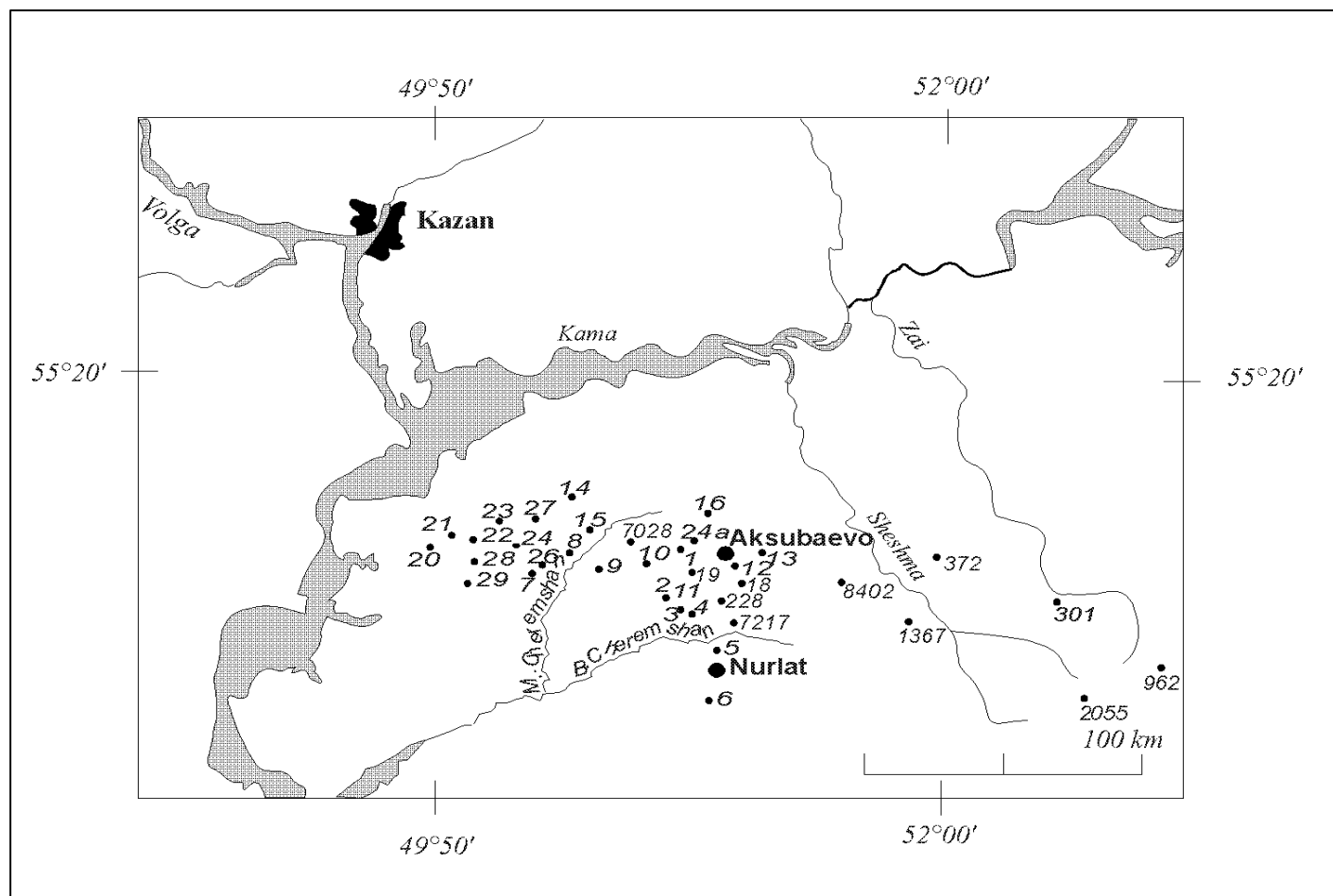
Figure 1. Map showing location of investigated wells.
