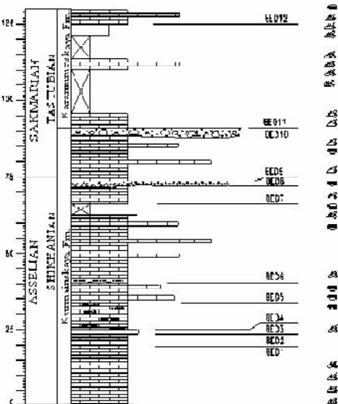
Figure 2. Stratigraphic column of section II and III, Kondurovsky, Russia. Conodont and fusulinid distribution indicated by \blacktriangle and \bullet symbols.
