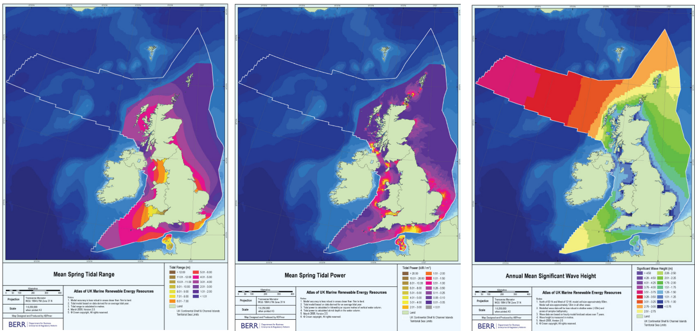
Figure 1: Mean Spring tidal range; Figure 2: Mean Spring tidal stream and Figure 3: Annual mean significant wave 13
