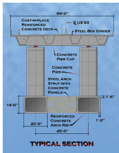
Fig. 3 - Typical Section
