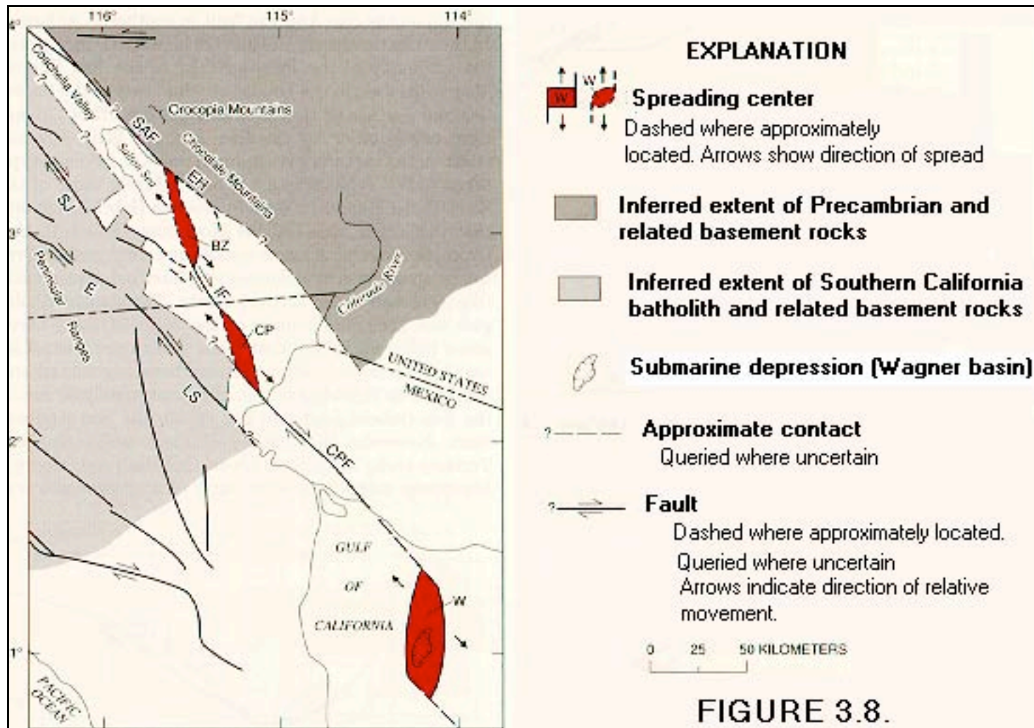
FIGURE 3.8: Salton Trough, showing major spreading centers and termination of the San Andreas fault. Spreading centers: BZ, Brawley seismic zone; CP, Cerro Prieto geothermal area; W, Wagner Basin. Major transform faults: CPF, Cerro Prieto; IF, Imperial; SAF, San Andreas. Other major faults: E, Elsinore; EH, East Highland Canal seismicity lineament; LS, Laguna Salada; SJ, San Jacinto.
